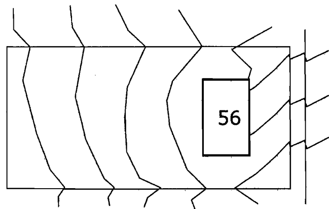
TYPICAL LOT GRADING W/REAR DRAINAGE NTS
